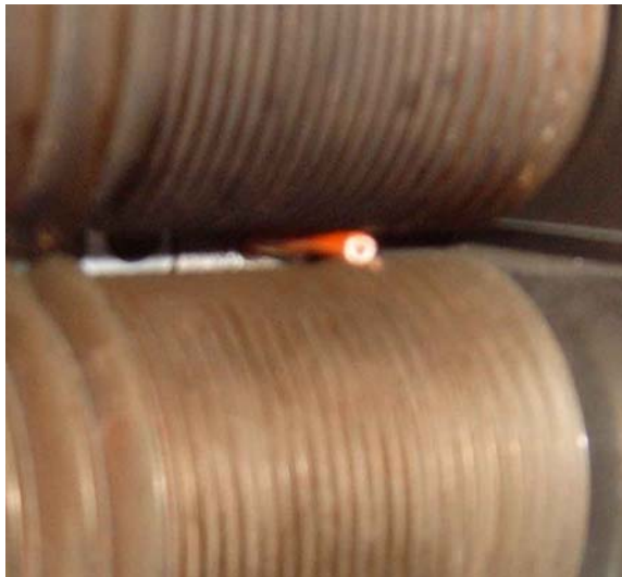
Figure 4-3, Wire between cutter blades.
