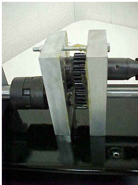
Figure 5-2 Spur Gears
