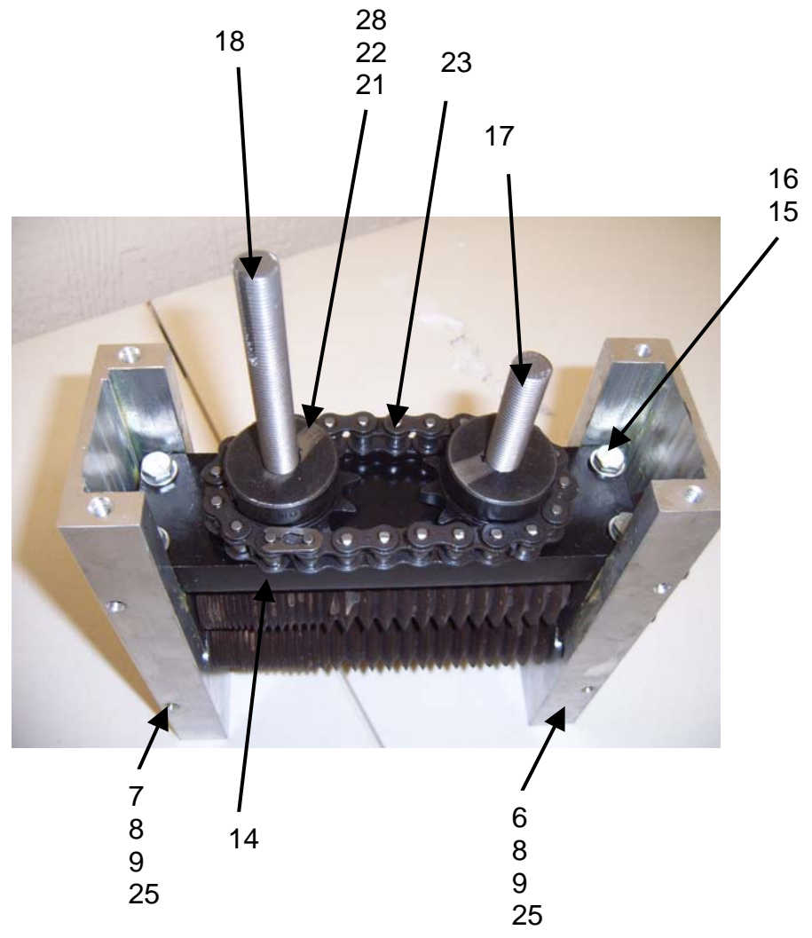
Figure 6-1, Cutter System (Model 1000)
