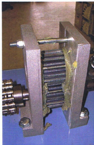
Figure 5-2 Spur Gears
