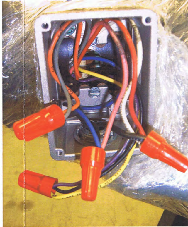
MOTOR WIRING 10 GA WIRE FROM STARTER (ITEM -65)
